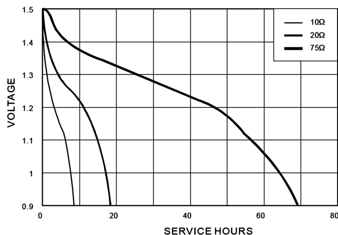
TYPICAL DISCHARGE CHARACTERISTICS AT 21\text{ }^{\circ}\text{C} ( 60 \pm 15\% RH)
